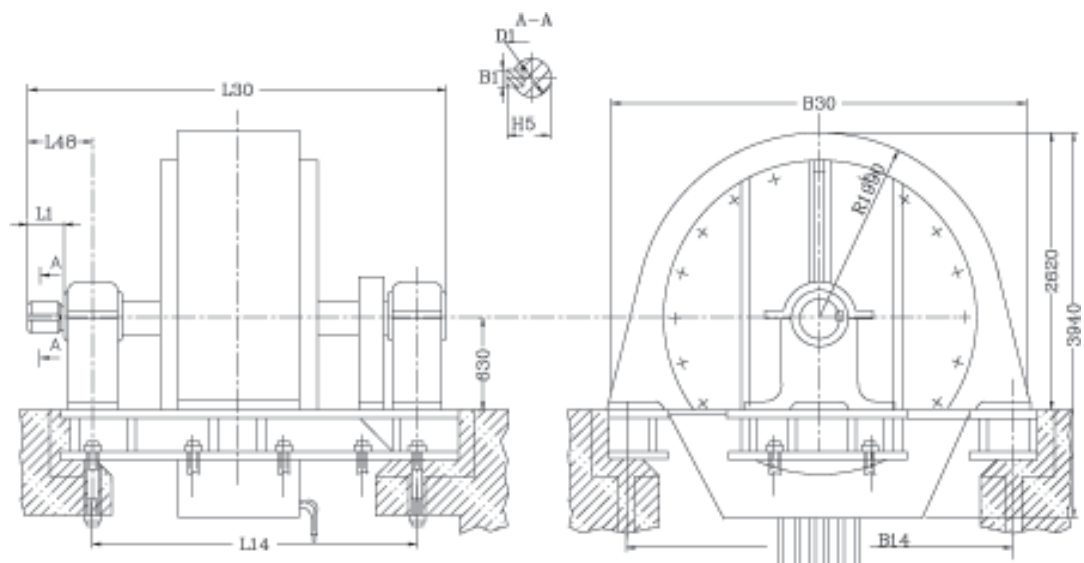
СДМ32-21-61,67,91
