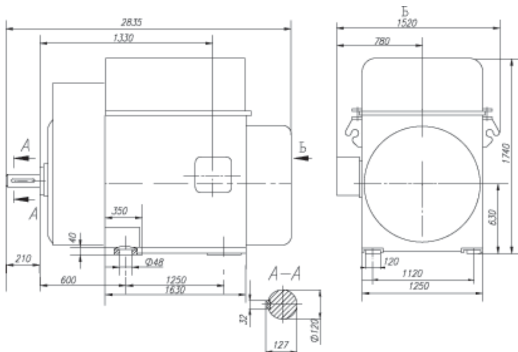
AOK-400-0,46-600T1
