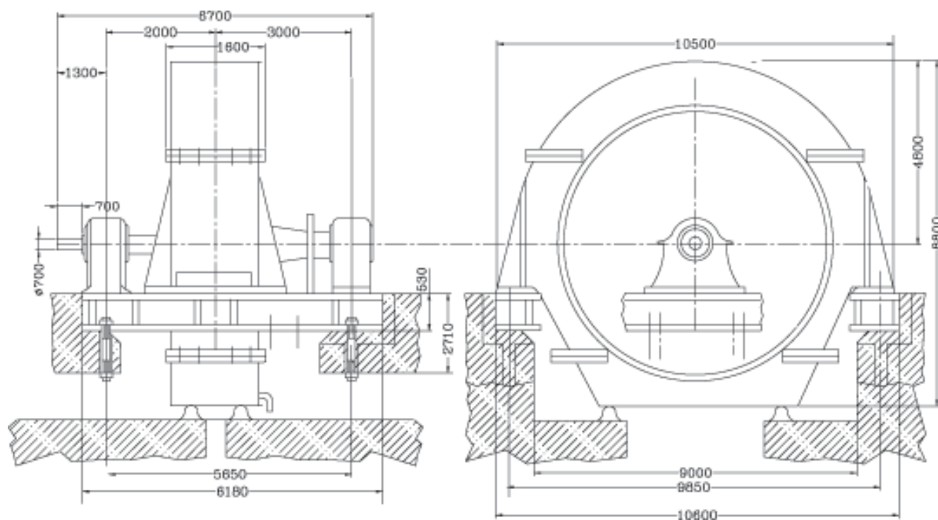
СДМ32-24-59-80
