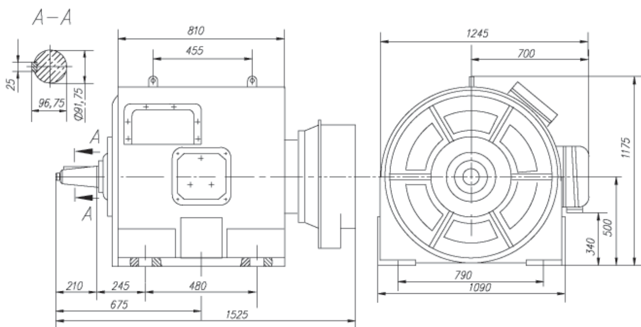
AKЭ-110-0,38-500
