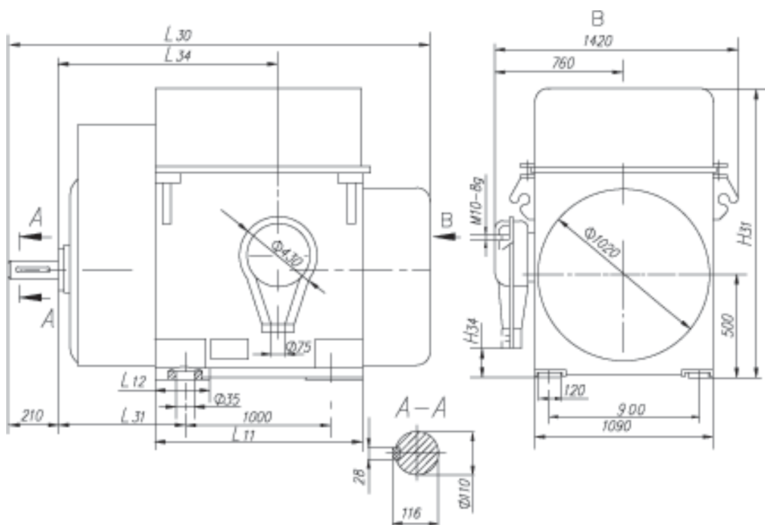
AOK-400-0,46-600T1
