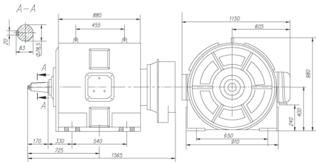
AKЭ-110-0,38-600
