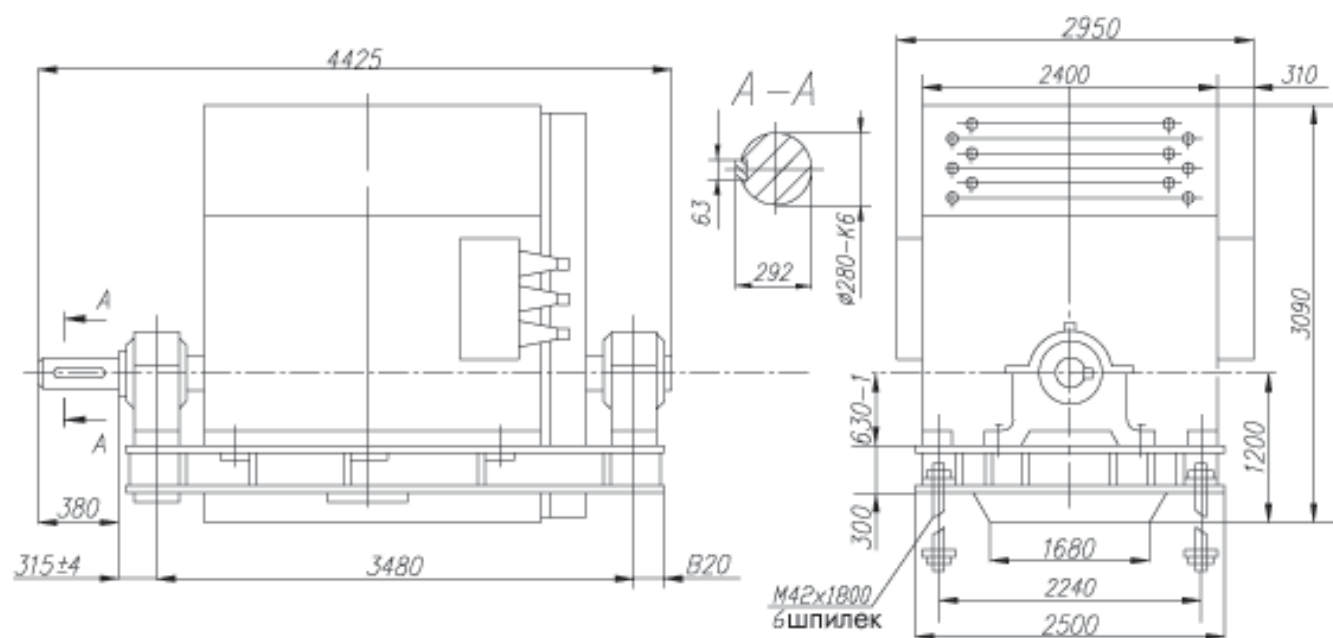
AO-3200-6-600УХЛ1
