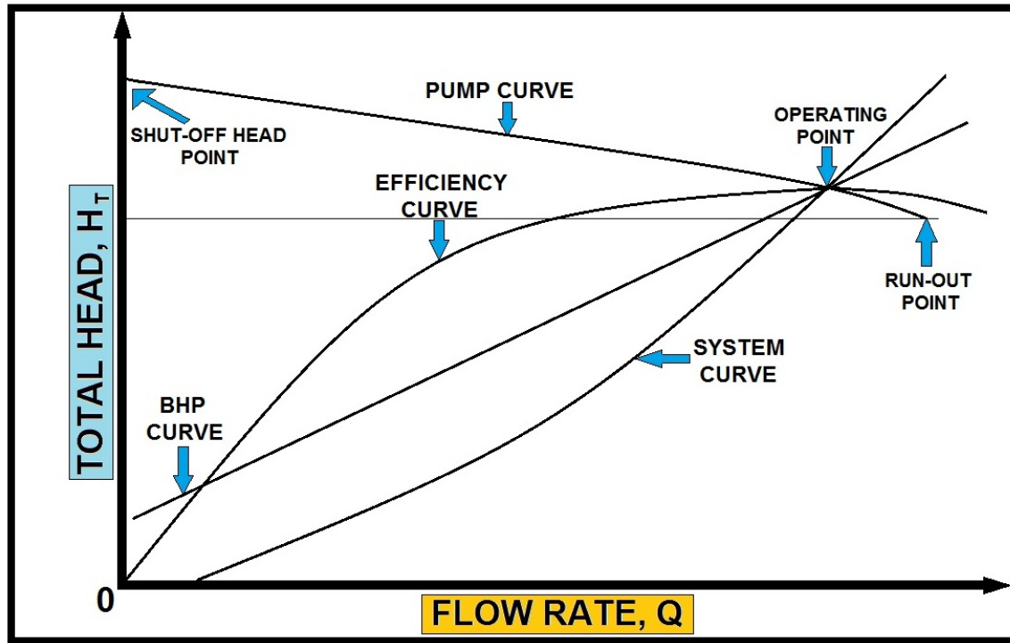
PUMP PERFORMANCE CURVE (CENTRIFUGAL PUMP)
