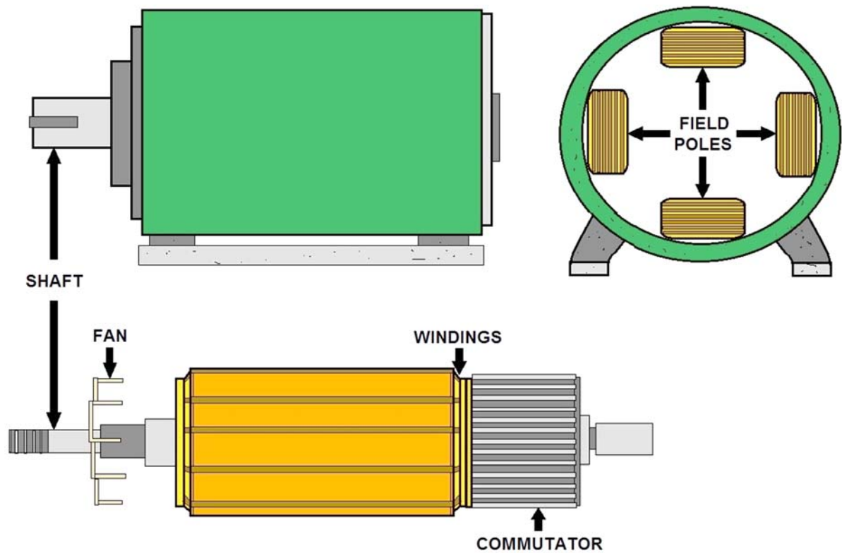
DC ELECTRIC MOTOR DIAGRAM
