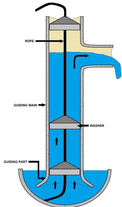
ROPE PUMP DESIGN
