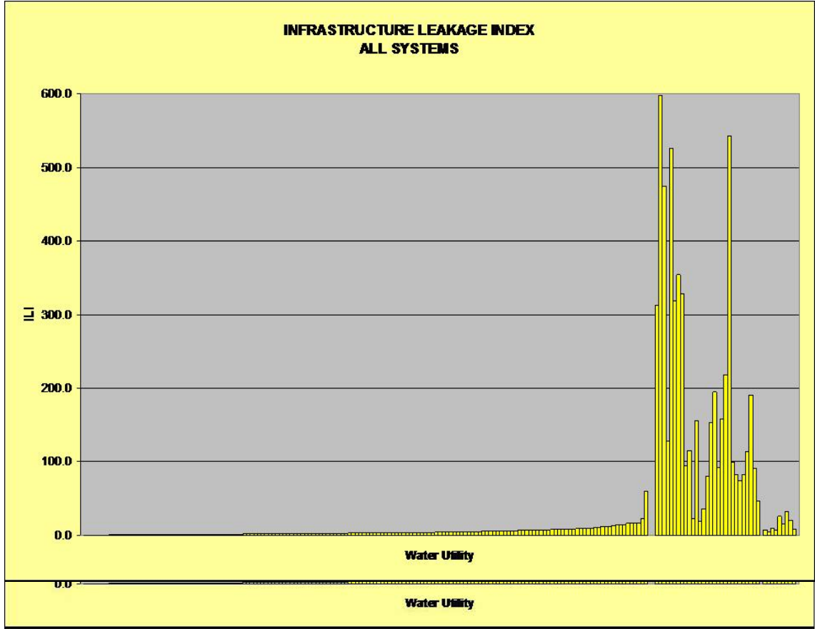
Figure 13: ILI for complete data set
