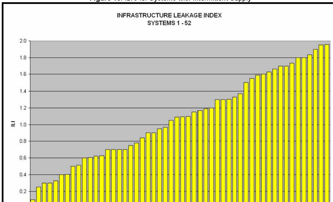
Figure 15: ILI's for Systems with Intermittent Supply
