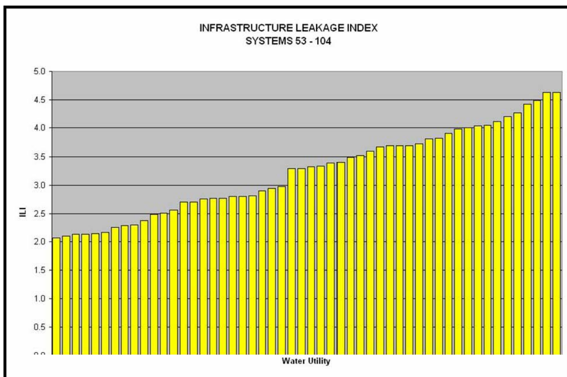
Figure 17: ILI's for utilities 53 to 104 in ascending order
