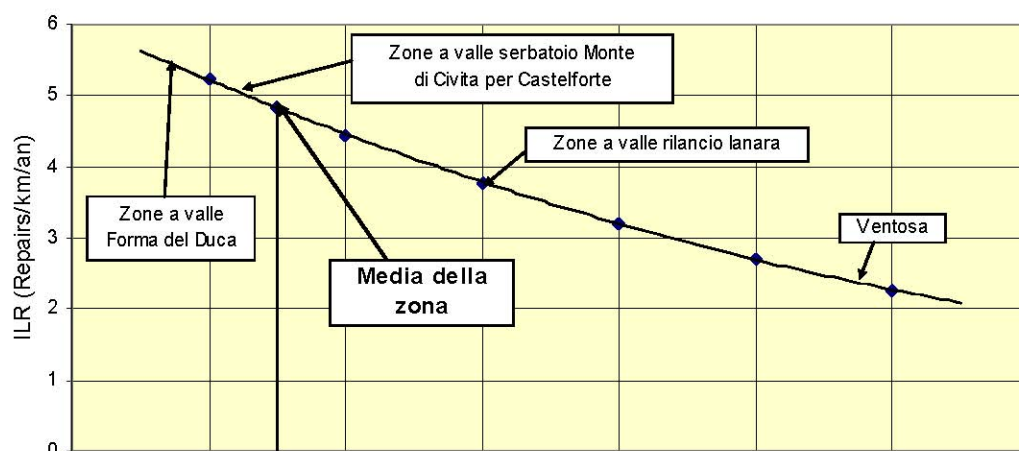
Economic linear repair ratio for ND100 pipes in SS Cosma e Damiano - Castelforte according to the different distribution areas
