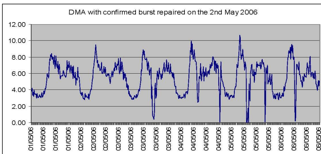
Graph 1.2 – Burst repaired on 02/05/2006
