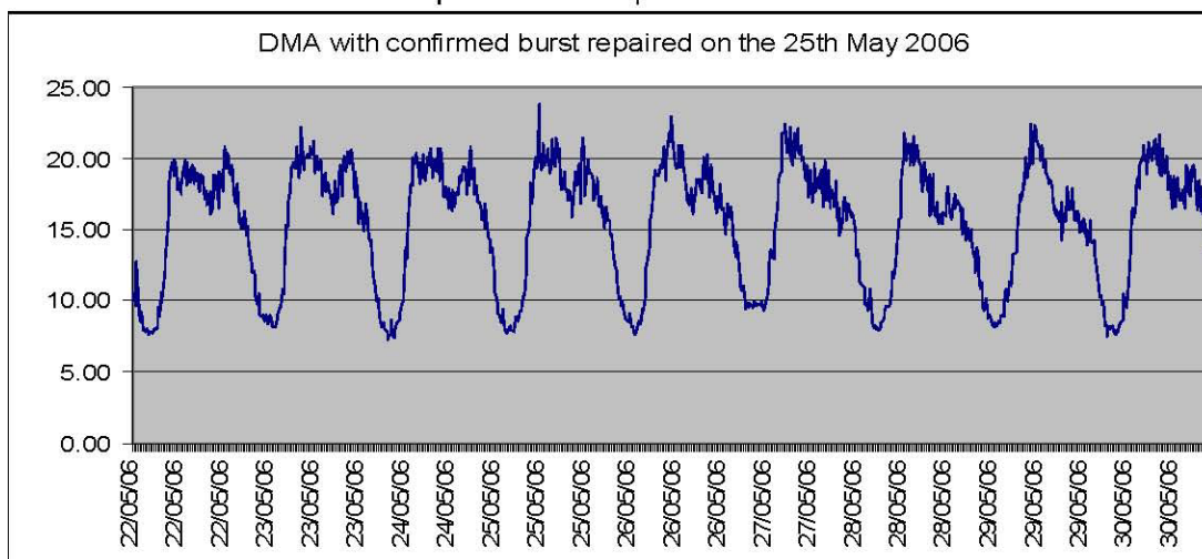
Graph 1.3 – Burst repaired 25/05/2006
