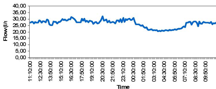
Daily flow pattern in DMA 100 (22.05.2007)
