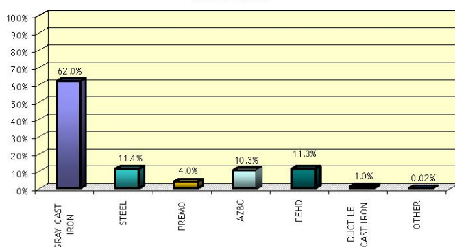
PERCENTAGE NETWORK DISTRIBUTION ACCORDING TO THE MATERIAL
