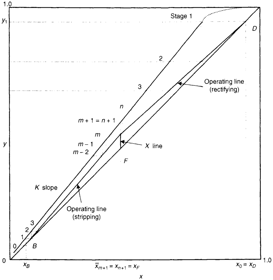
Figure 4.7 Graphical schematic representation for the McCabe-Thiele method as applied to membrane separations, where X = 1 .
