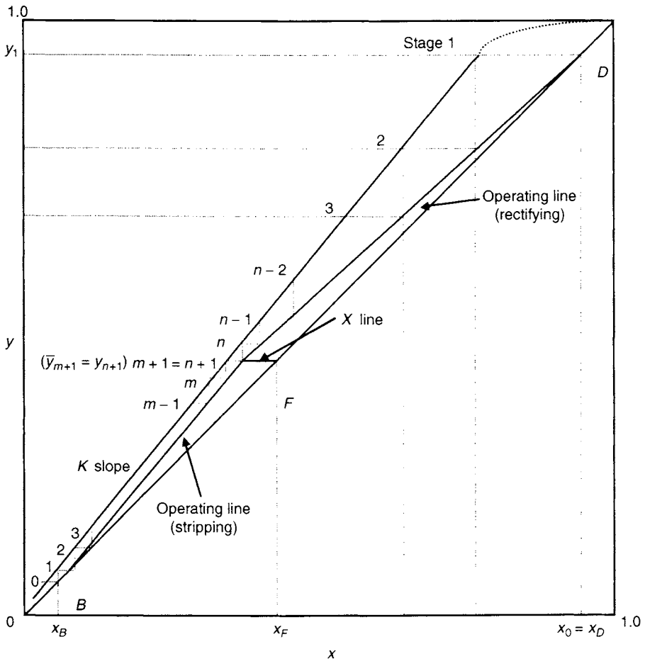
Figure 4.8 Graphical schematic representation for the McCabe-Thiele method as applied to membrane separations, where X = 0 .
