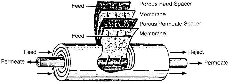
Figure 1.3 Spiral-wound membrane. (Source: Bravo et al. 6 )
