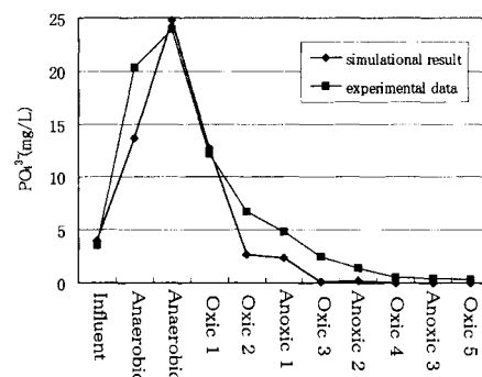
Figure 10. Experimental and simulated \text{PO}_4^{3-} concentration in each stage in multiple stages EBNR process ( Q_1 : Q_2 : Q_3 = 0.7 : 0.2 : 0.1 )
