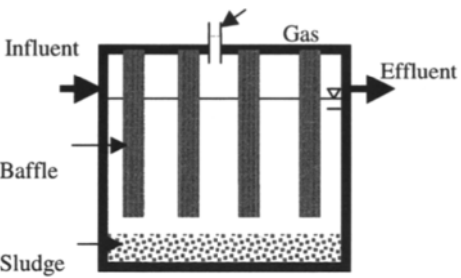
Figure 2. Reactor B – Anaerobic baffled
