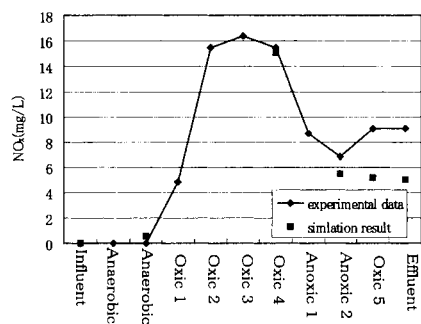
Figure 5. Experimental and simulated \text{NO}_x concentration in each stage in AOA process ( Q_1 : Q_2 = 0.8 : 0.2 )
