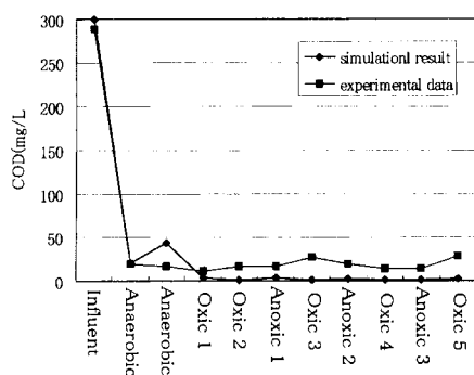
Figure 3. Experimental and simulated \text{COD}_s concentration in each stage in AOA process ( Q_1 : Q_2 = 0.8 : 0.2 )
