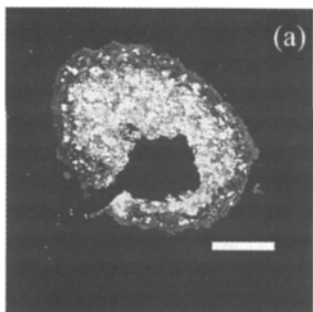
Figure 3. FISH image of the biofilm in Reactor C, organic wastewater. (a) FISH image of a cross section of the entire biofilm, bar = 200 \mu\text{m} and (b) magnified image showing each cell individually, bar = 20 \mu\text{m} . White part shows ammonia-oxidizing bacteria detected by both FITC-labeled probe NEU23a and Cy5-labeled probe EUB338. The gray part shows other bacteria detected only by the probe EUB338 (heterotrophs).
