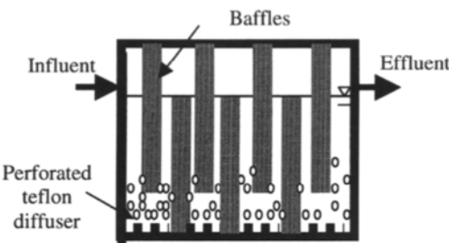
Figure 1. Reactor A – Aerobic baffled
