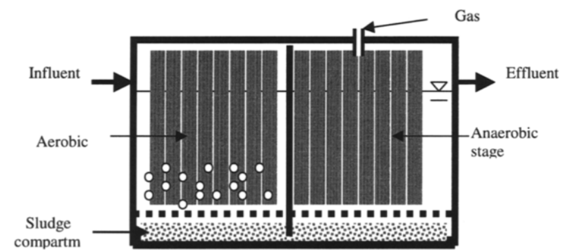
Figure 3. Reactor C – Aerobic-anaerobic baffled
