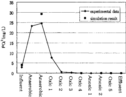
Figure 6. Experimental and simulated \text{PO}_4^{3-} concentration in each stage in AOA process ( Q_1 : Q_2 = 0.8 : 0.2 )
