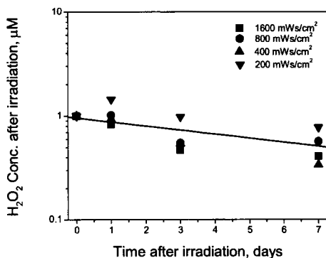
Figure 4. Decay of UV-irradiation-induced \text{H}_2\text{O}_2 with time. The best fit curve is drawn for the data of 800-mWs/cm 2 UV-dose.
