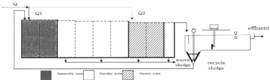
Figure 1. Pilot plant diagram of AAO process
