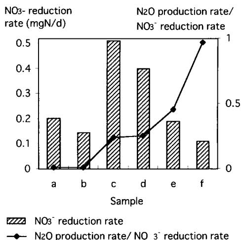
Figure 7. \text{NO}_3^- -N reduction rate (column) and the ratio of the \text{N}_2\text{O} production rate to \text{NO}_3^- -N reduction rate (N _2\text{O} emission ratio, line)
