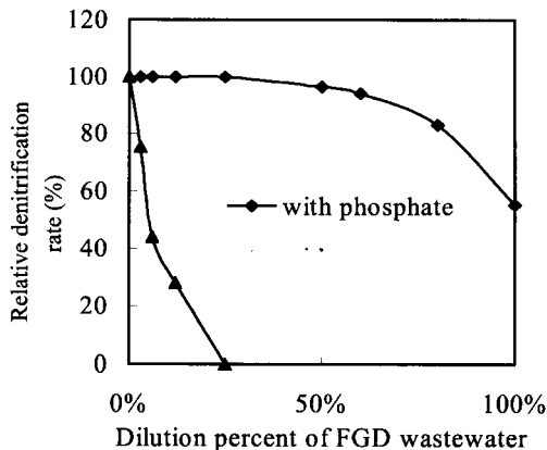
Figure 5. Effect of nutrient addition on denitrification rate
