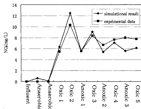
Figure 9. Experimental and simulated \text{NO}_x concentration in each stage in multiple stages EBNR process ( Q_1 : Q_2 : Q_3 = 0.7 : 0.2 : 0.1 )
