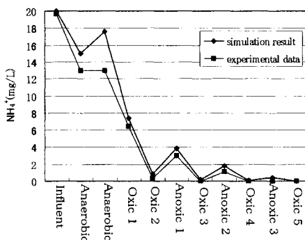
Figure 8. Experimental and simulated \text{NH}_4^+ concentration in each stage in multiple stages EBNR process ( Q_1 : Q_2 : Q_3 = 0.7 : 0.2 : 0.1 )
