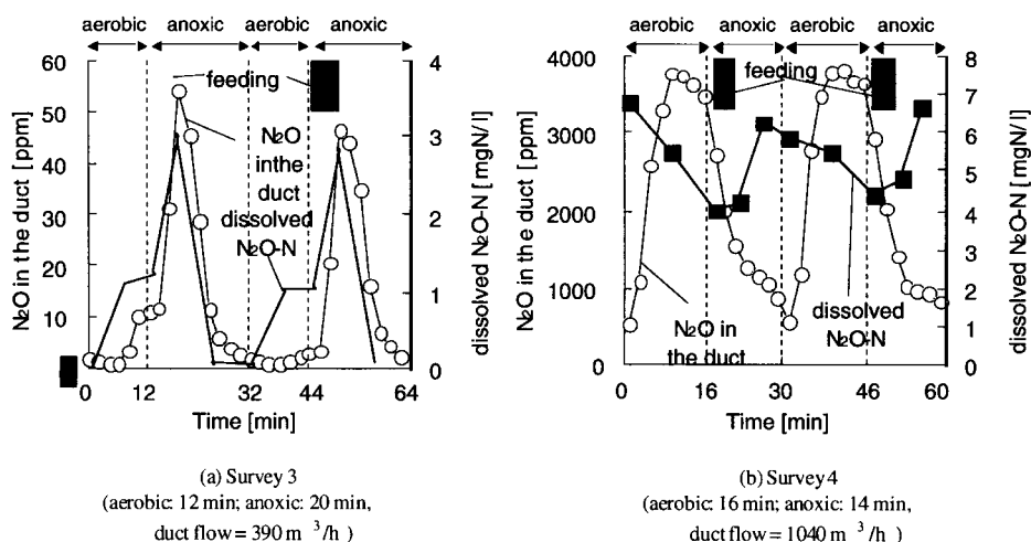
Figure 4. \text{N}_2\text{O} concentrations in the duct of the intermittent aeration tank and dissolved in the mixed liquor [12].
