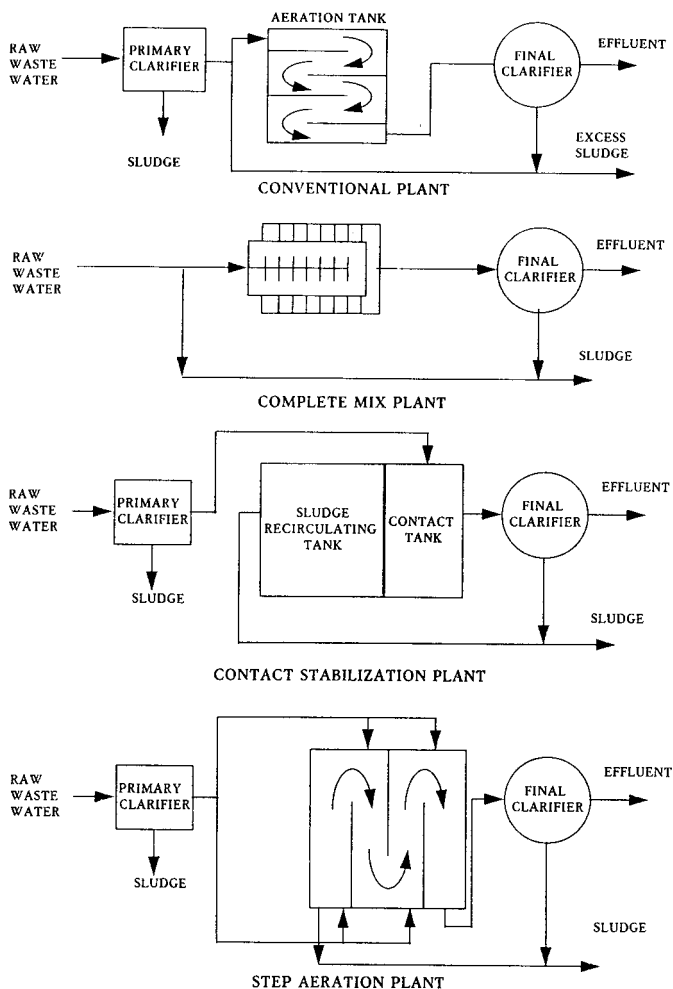
Figure 3. Variations of the activated sludge process.
