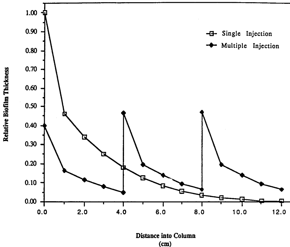
Figure 10. Relative biofilm thicknesses comparing single and multiple nitrate injections.
