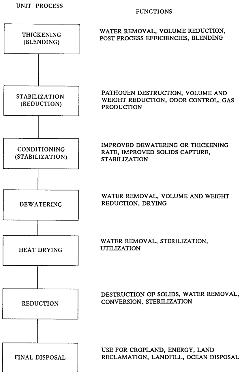
Figure 9. Sludge treatment processes and their functions.
