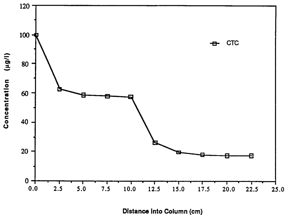
Figure 12. Profile showing additional secondary utilization of CTC after SOC is added by a second injection at 10 cm.
