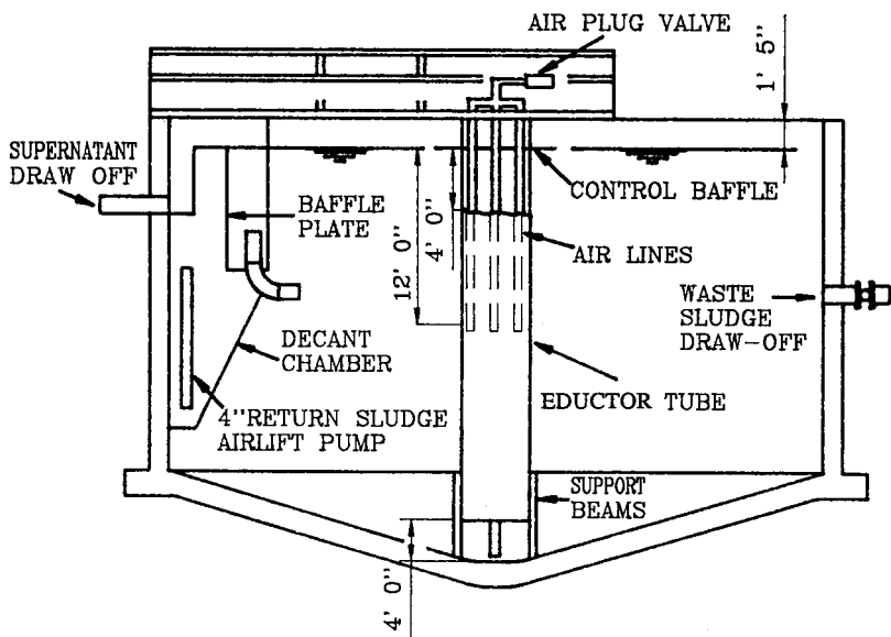
Figure 4. Typical aerobic circular digester.
