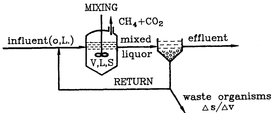
ANAEROBIC ACTIVATED SLUDGE PROCESS
