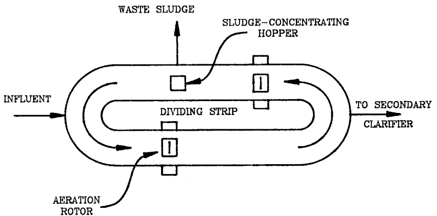
Figure 5. Oxidation ditch flow diagram.
