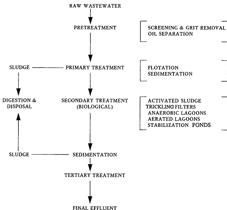
Figure 10. Typical wastewater treatment sequence incorporating biological treatment processes.
