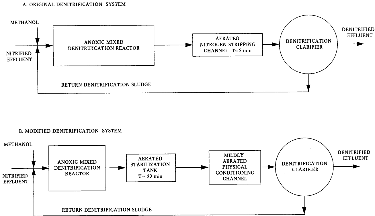
Figure 4. Suspended growth denitrification systems using methanol.
