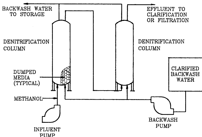
Figure 3. Typical process schematic for submerged high porosity media columns.
