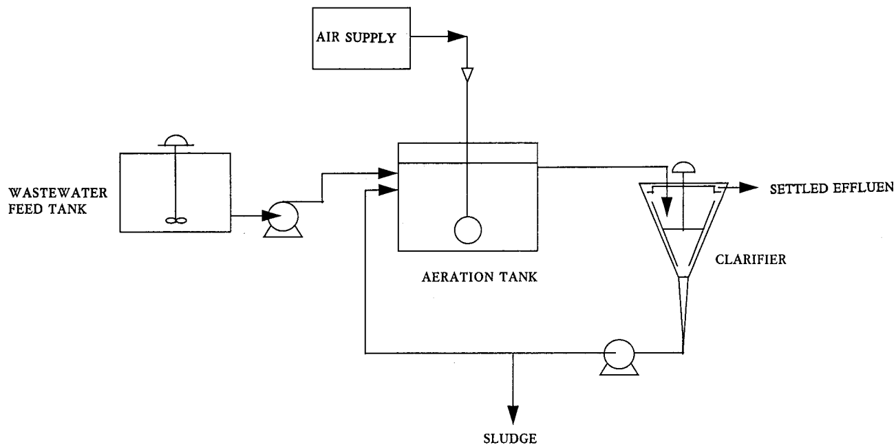
Figure 3. Schematic of a continuous-flow aeration unit.
