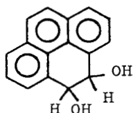
Ring oxidation products
