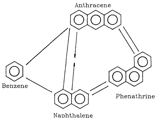
Figure 6. Proposed relationship between benzene and the PAHs used in the study.
