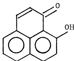
4 hydroxyperinaphthenone
