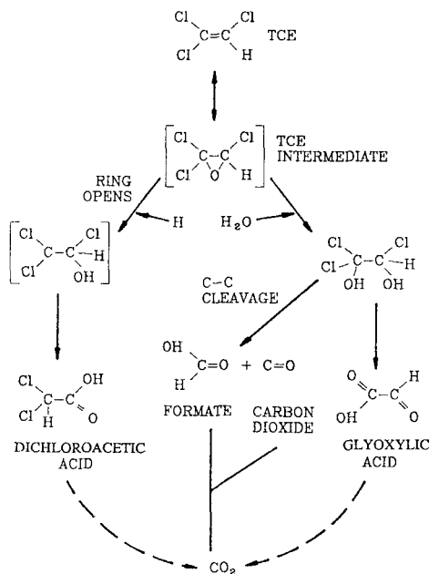
Figure 3. Reprinted from: TCE Degradation by a Methane-Oxidizing Bacterium. Little et al., App & Env Mic , April 1988.
