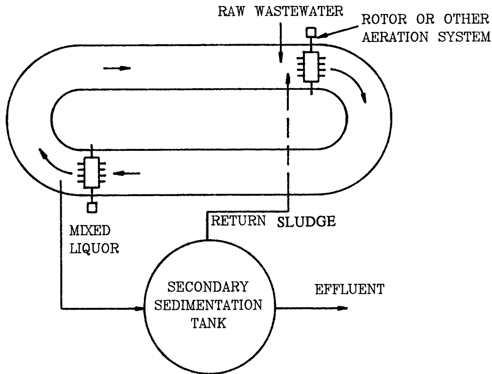
Figure 9. Pasveer ditch or endless channel system for nitrogen removal.
