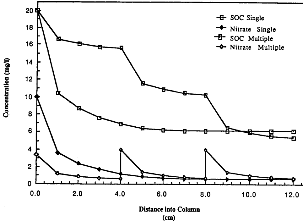
Figure 9. SOC and nitrate profiles for one and three injections of \text{NO}_3^- .
