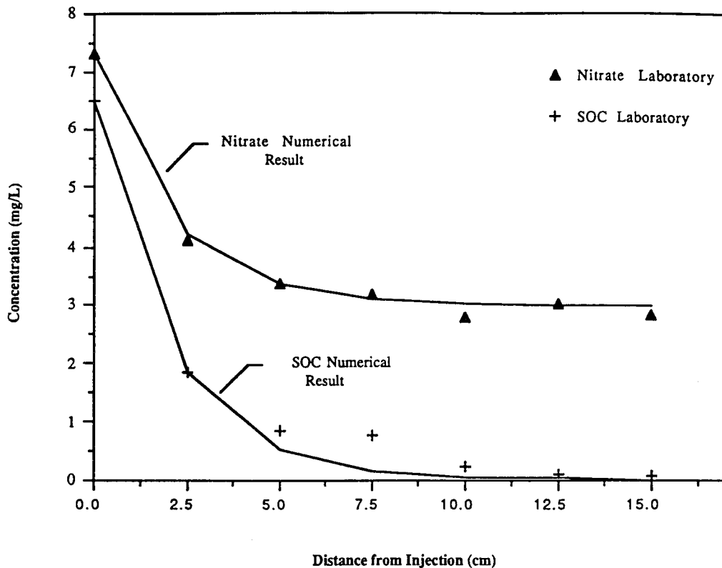
Figure 2. Comparison of laboratory and numerical results for the one-BAZ column. Zero distance indicates the injection port.
