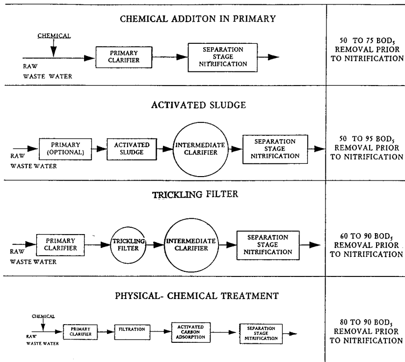
Figure 1. Pretreatment alternatives for separate stage nitrification.
