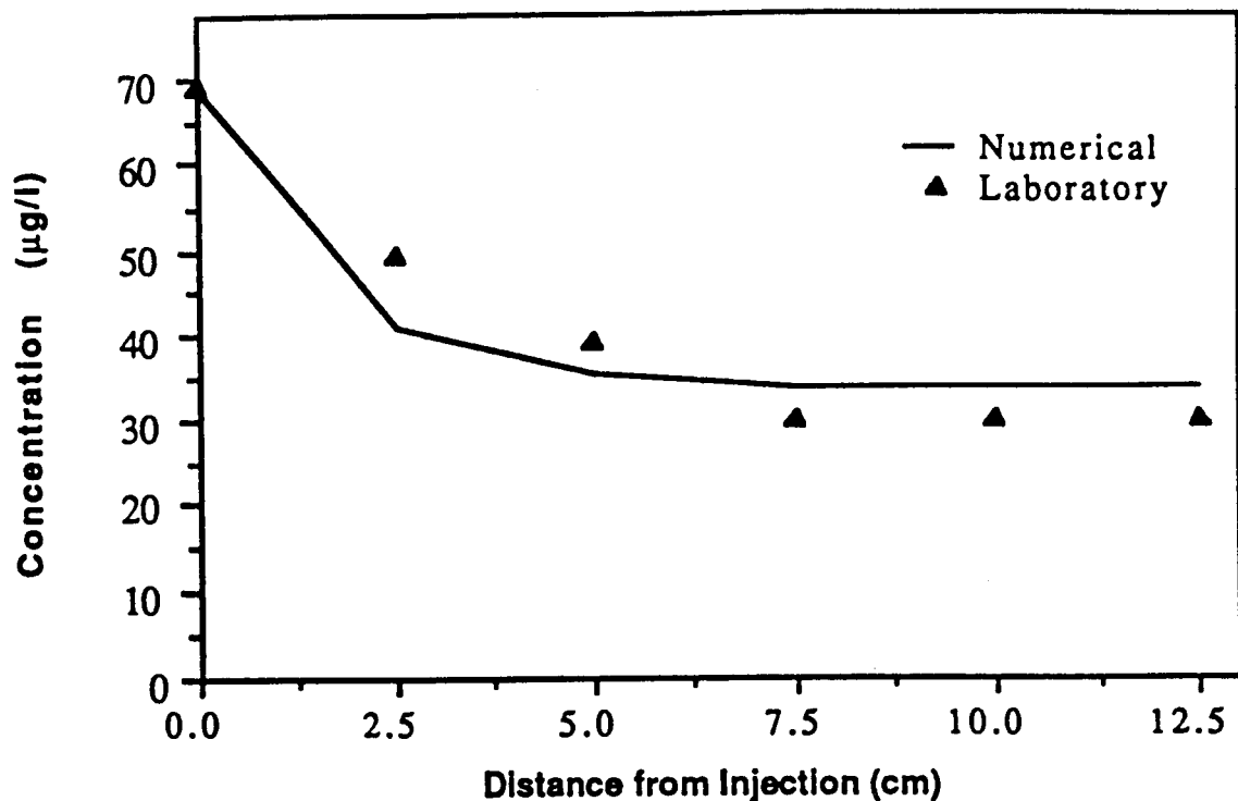
Figure 5. Prediction of the CTC profile at a detention time of 125 min. and with k = 0.030 \mu\text{g}/\text{mg cell-day} and K_s = 4.5 \mu\text{g}/\text{l} .
