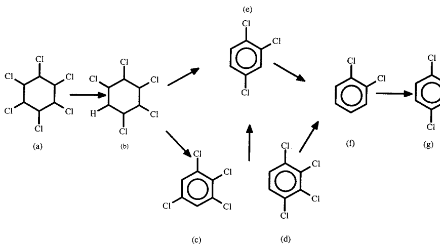
Figure 11. Proposed initial steps of alpha-HCH degradation under aerobic conditions in a slurry of contaminated soil. (A) Alpha-HCH; (B) PCHH; (C) 1,2,3,5-TeCB; (D) 1,2,4-TCB; (E) 1,2,4-DCB; (F) 1,2-DCB; (G) 1,4-DCB. Reprinted from Bachman et al., App & Env Mic , vol. 54, Feb. '88, p. 553.
