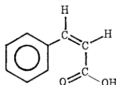
4 hydroxyperinaphthenone
