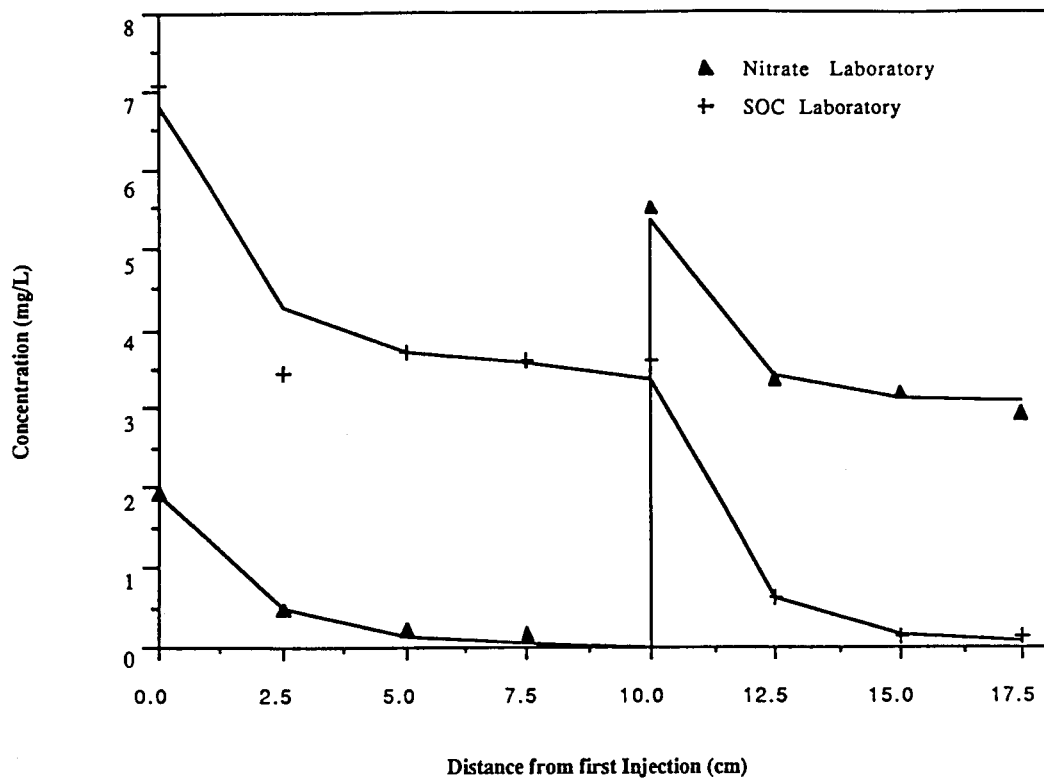
Figure 3. Comparison of laboratory and numerical results for the two-BAZ column. Nitrate injections are at 0.0 and 10.0 cm. Lines represent model prediction.
