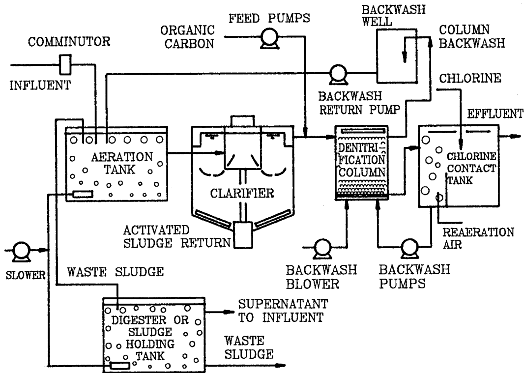
Figure 2. Nitrification-denitrification flow sheet utilizing low porosity fine media in columns.
