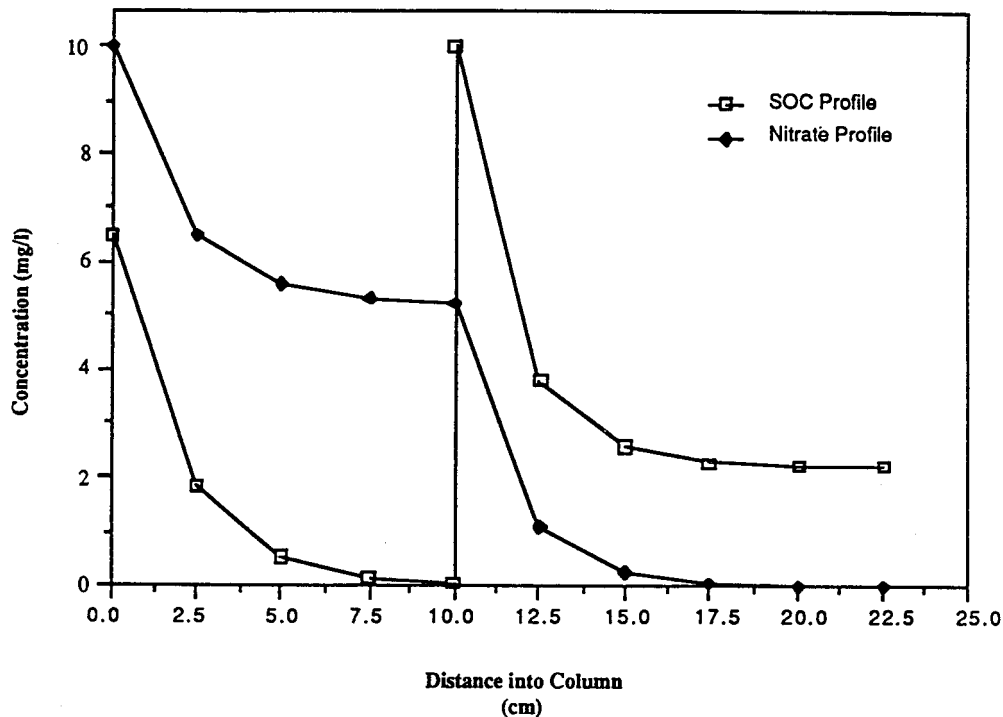
Figure 11. Profiles of SOC and nitrate after being injected alternately.
