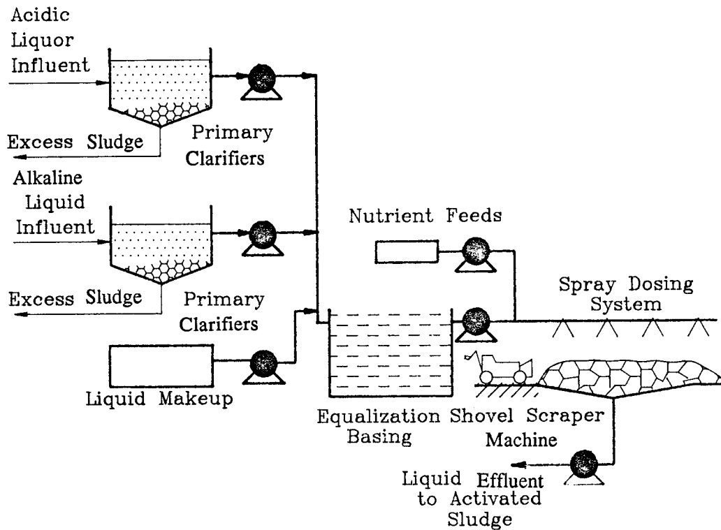
Figure 1. Biochemical compost bed system flow diagram.
