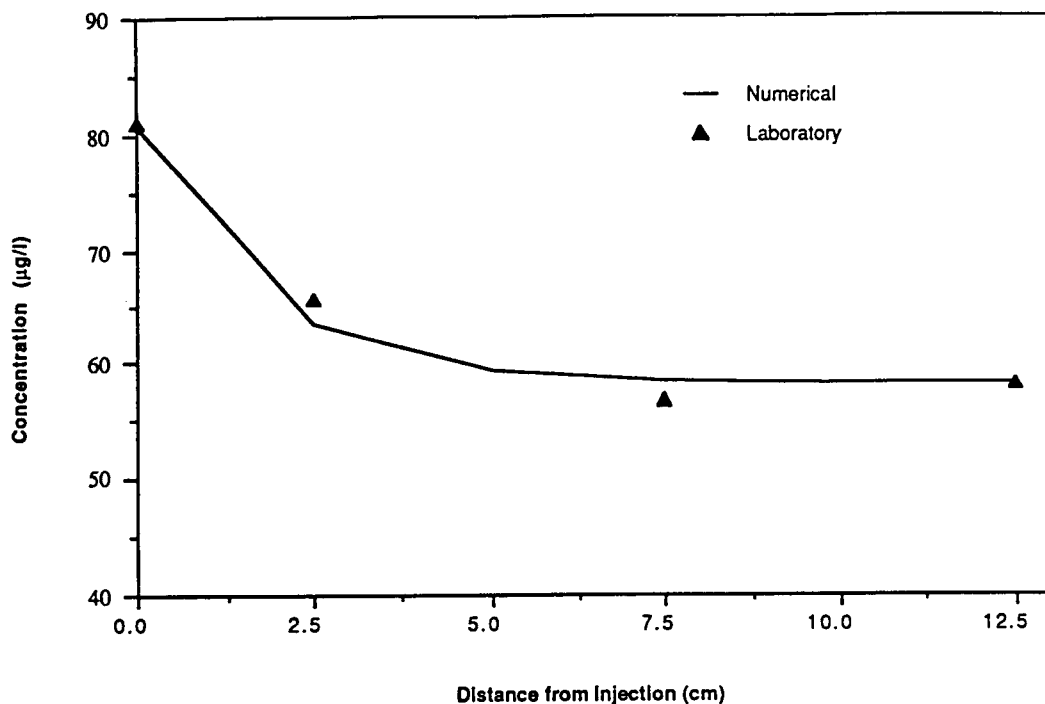
Figure 4. Numerical curve fit to the CTC profile at a detention time of 50.0 min. The k and K_s are 0.030 \mu\text{g/mg cell-day} and 4.5 \mu\text{g/l} , respectively.
