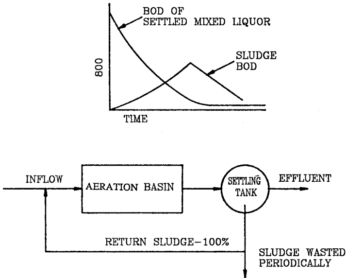
Figure 4. Extended aeration activated sludge.
