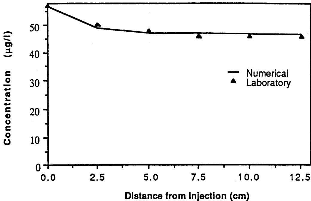
Figure 7. Numerical fit to the BF profile at a detention time of 125 min. The k and K_s are 0.013 \mu\text{g/mg cell-day} and 9.5 \mu\text{g/l} , respectively.
