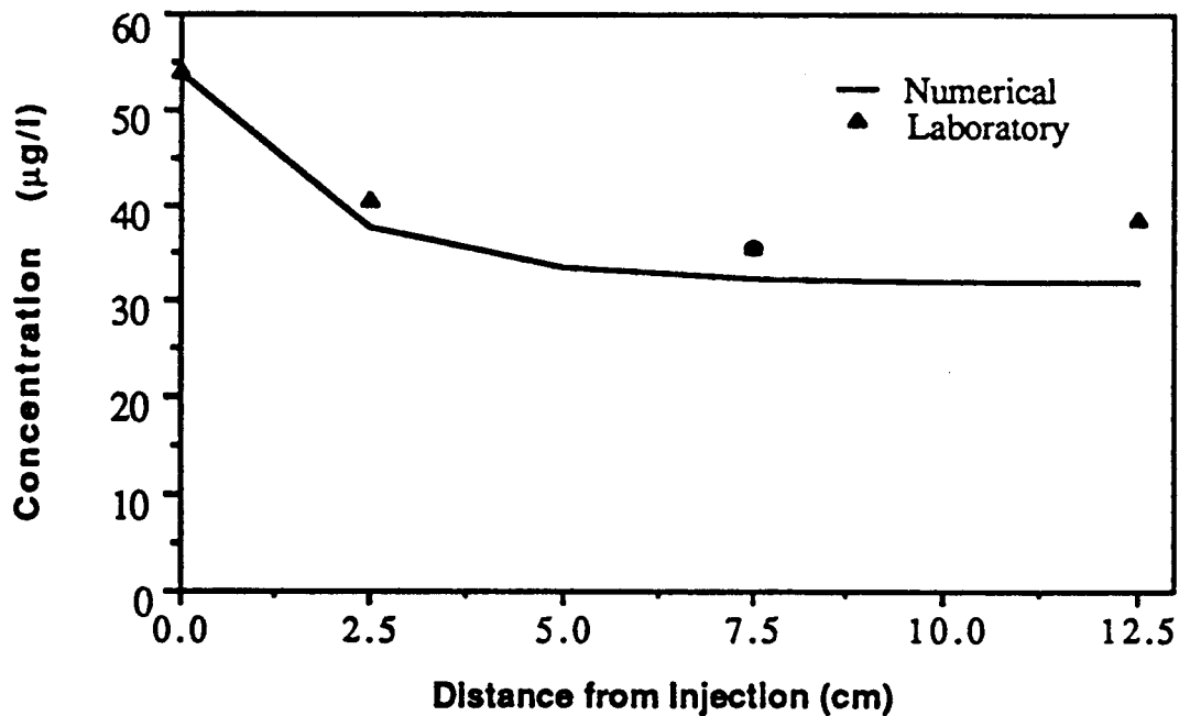
Figure 8. Prediction of the BF profile at a detention time of 500 min. and with k = 0.013 \mu\text{g/mg cell-day} and K_s = 9.5 \mu\text{g/l} .
