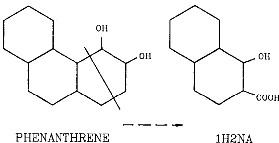
Figure 9. Phenanthrene degradation.
