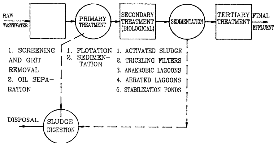
Figure 1. Typical wastewater treatment sequence.
