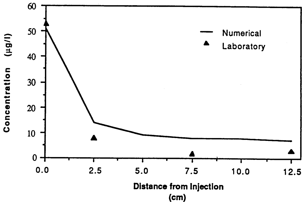
Figure 6. Prediction of the CTC profile at a detention time of 500 min. and with k = 0.030 \mu\text{g/mg cell-day} and K_s = 4.5 \mu\text{g/l} .
