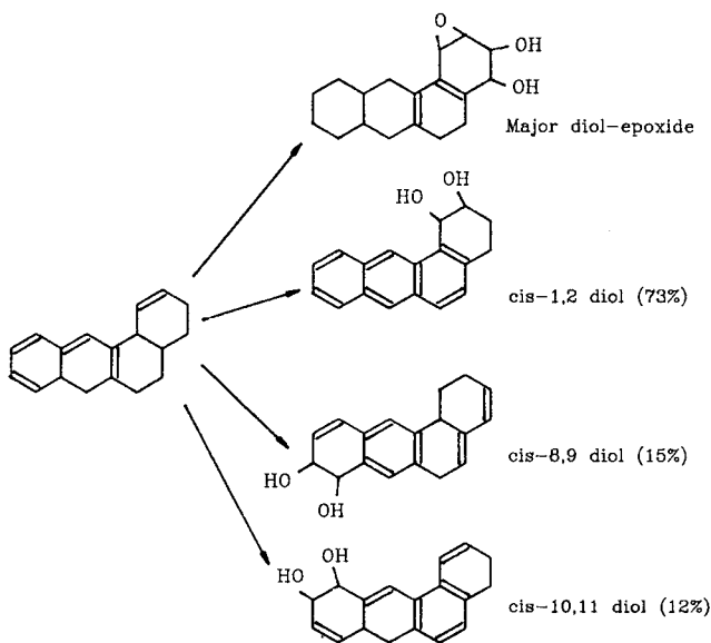
Figure 7. Chemical transition structure.
