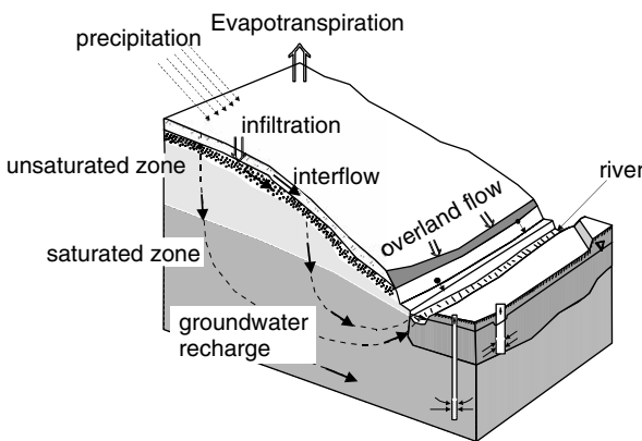
Figure 4.2. Block of a landscape with the respective run-off components
