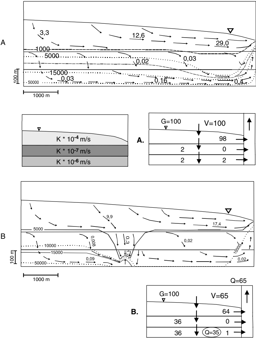
Figure 2.10. Flow lines (arrows), apparent flow velocities of the groundwater (m/day) and age distribution (years) in the groundwater (dotted lines) at a certain hydraulic conductivity distribution (m/s) in the aquifer systems. A. Without, B. with 35% of groundwater exploitation from the passive groundwater recharge zone
