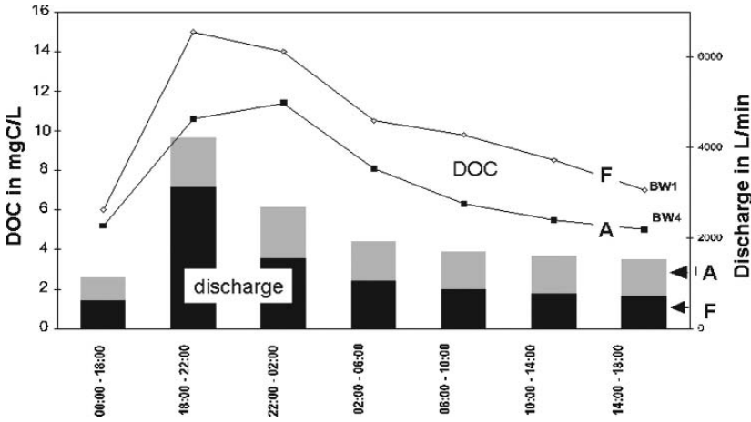
Figure 5.4. DOC in surface discharge during a discharge event in Tertiary sediments of the Molasse basin in south Germany (Scheuern area); F = 100% forest area, 0.45 km 2 in size A = 95% agricultural area and 5% forest area, together 0.74 km 2 in size
