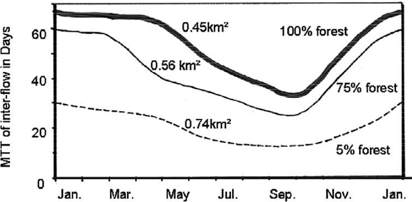
Figure 4.4. Seasonal changes of the mean turn-over time (MTT) of inter-flow in Tertiary sediments of south Germany (Scheyern). Catchment sizes are similar, but forest cover is changing
