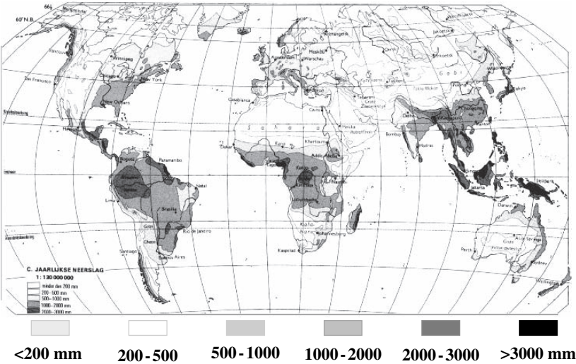
Figure 2.5. The global pattern of annual precipitation
