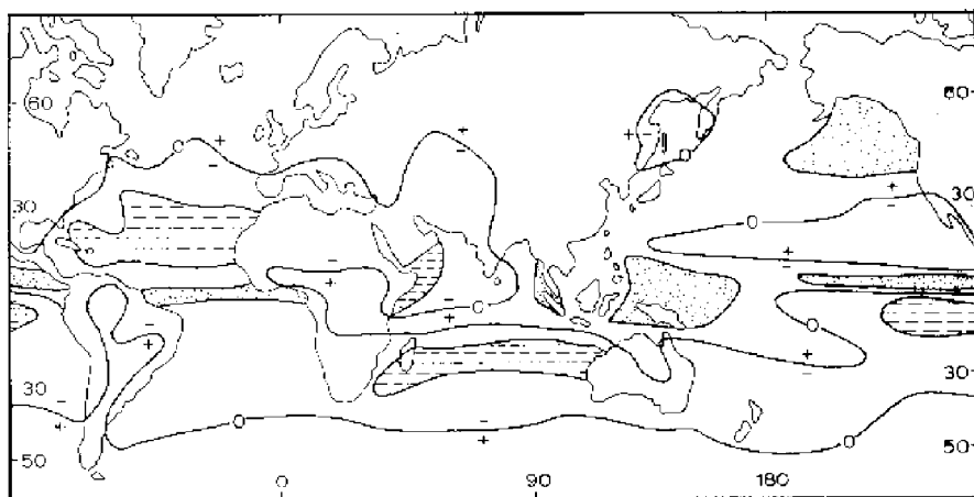
Figure 2.4. Precipitation/evaporation ratios exceeding (+) or remaining below (–) mean global ratio. Stippled areas: precipitation excess >100 \text{ mm/year} ; dashed areas: evaporation excess >100 \text{ mm/year} (Lisitzin, 1971)
