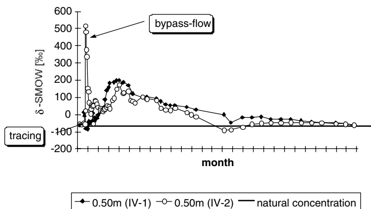
Figure 3.8. Quick and slow tracer-break-through (TBT) from a tracer experiment in Quaternary loess of the Scheyern test site in south Germany. Deuterium ( ^2\text{H} ) was used as a tracer and sampling was performed continuously at two points in 0.5 m b.g.s., which have been 50 cm distant from one another. Preferential-flow is indicated by a positive pulse at the beginning and many negative pulses during the break through of the tracer test
