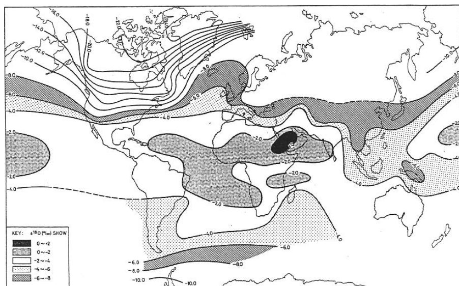
Figure 4.28. World-wide distribution of the annual means of \delta^{18}\text{O} in precipitation (Yurtsever & Gat, 1981)
