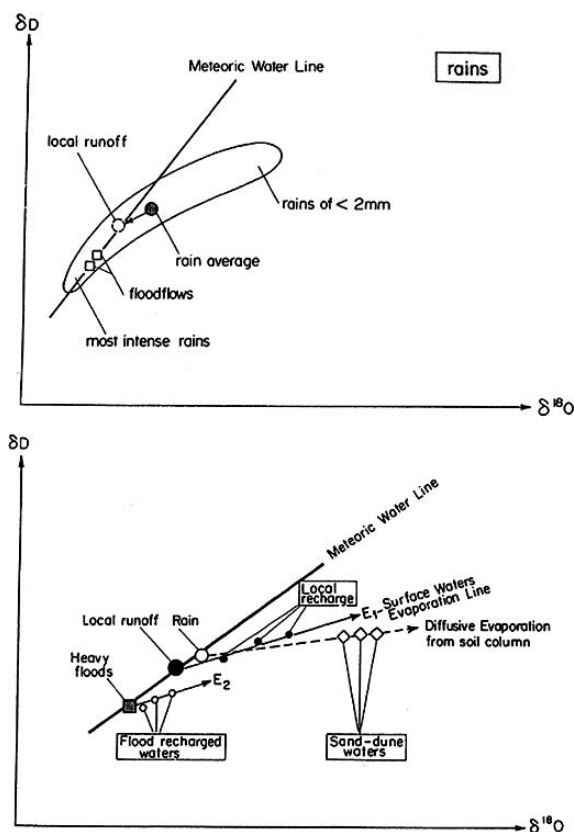
Figure 5.12. Isotope relationship between the mean desert showers and discharge
