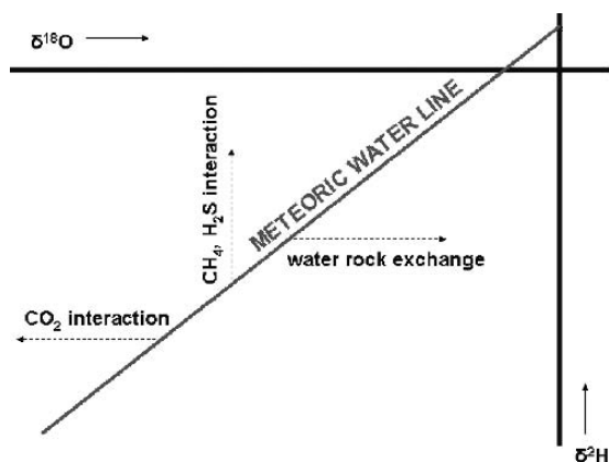
Figure 4.15. Changes of the stable water isotope signature by special water/rock/gas interactions in the subsurface
