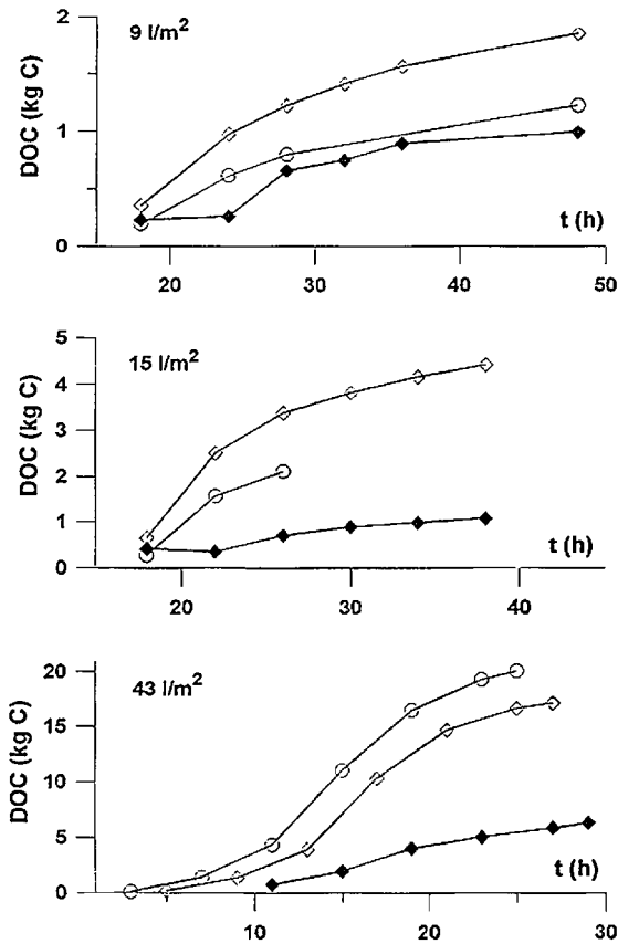
Figure 5.5. DOC concentrations in surface discharge during low and high rain amounts, shown for catchments with different vegetation covers (circles = mixed forest and agro-land, open rhomb = forest, black rhomb = grassland)
