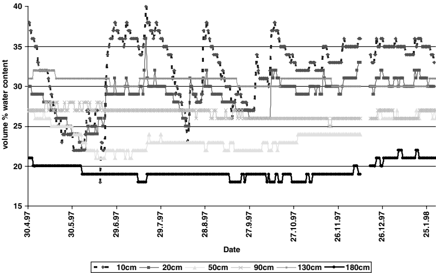
Figure 4.11. Changes of water contents in depths between 10 cm (black with great variations) and 180 cm (black with little variations), measured during one vegetation period, followed by a bare soil period in gravely sands of Scheyern, South Germany. Measuring period April 30, 1997, to January 25, 1998
