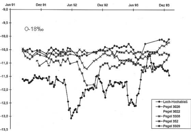
Figure 4.34. ^{18}\text{O}/^{16}\text{O} ratios in the groundwater remote and close to the river Lech, Germany, from 2 weeks sampling. Data from P. Trimborn, GSF-Institute of Hydrology, Neuherberg, Germany
