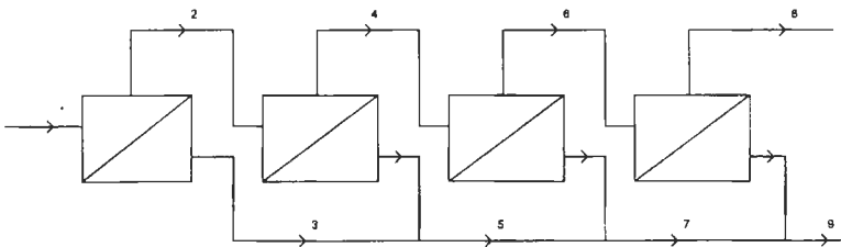
Figure 2.19 Retentate flow (streams 2, 4, 6 and 8) through a reverse osmosis module
