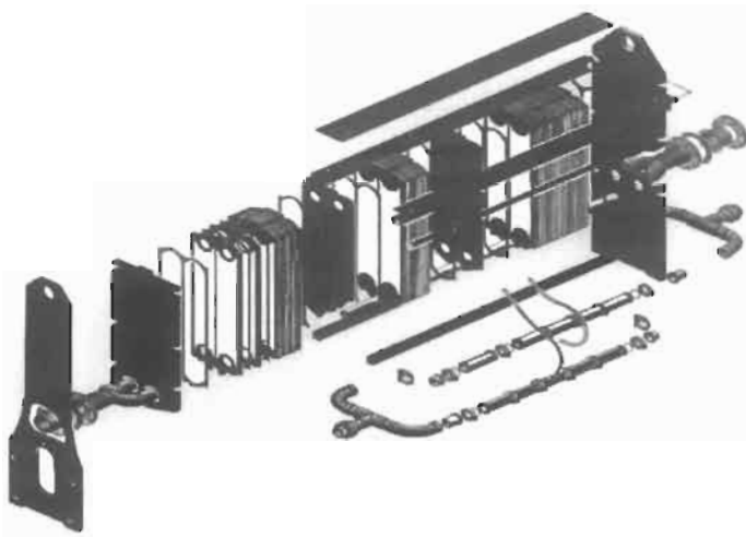
Figure 2.7 Rhodia Orelis PLAIDE MF membrane module
