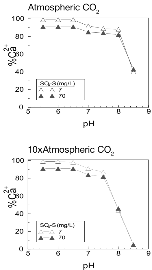
Figure 9.1. Removal of calcium from solution as calcite with increasing pH, carbon dioxide pressure and sulfate content of water. Composition of the drinking-water: Ca, 16 mg/l; Mg, 1.6 mg/l; SO 4 , either 7 or 70 mg/l; Cl, 35 mg/l; PO 4 , 1 mg/l; CO 2 , either 35.5 Pa (upper panel) or 355 Pa (lower panel).
